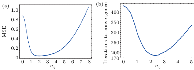
Fig. 3. (a) The MSE and (b) the number of iterations required for convergence versus the injected noise intensity \sigma_\eta . The threshold parameter of the bisquare function in Eq. (16) is set to \gamma = 2 , and the background noise \omega_n follows a standard Cauchy distribution with intensity \sigma_\omega = 1 .
