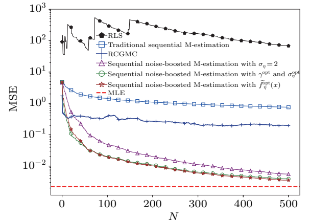
Fig. 2. Convergence curves of the MSE for the RLS algorithm, the traditional sequential M-estimation algorithm, the RCGMC algorithm, and the sequential noise-boosted M-estimation algorithm. For the sequential noise-boosted M-estimation algorithm, three cases are considered: a fixed threshold \gamma = 2 with Gaussian noise intensity \sigma_\eta = 2 ; the approximate optimal noise PDF \tilde{f}_\eta^{\text{opt}}(x) defined in Eq. (20); and the optimized parameters \gamma^{\text{opt}} = 8.76 and \sigma_\eta^{\text{opt}} = 2.6762 . The approximate optimal noise PDF \tilde{f}_\eta^{\text{opt}}(x) with K = 3 Delta kernel functions is determined by parameters v_1 = 0.3512 , v_2 = 0.1723 , v_3 = 0.4765 , \mu_1 = 1.1609 , \mu_2 = 3.0505 , \mu_3 = 0.6393 , and \gamma = 6.9282 via Bayesian optimization.
