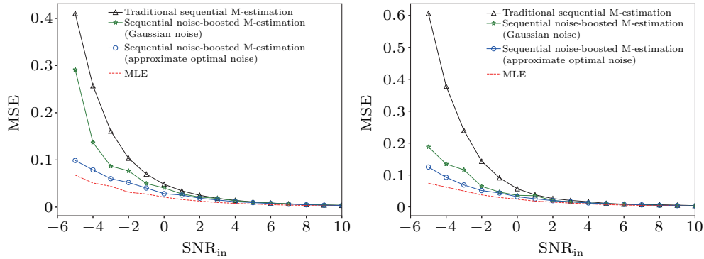
Fig. 6. Performance comparison of the sequential noise-boosted M-estimation algorithm with optimal added Gaussian noise (☆) and optimal added noise distribution in Eq. (20) with K = 4 (○), traditional sequential M-estimation algorithm (△), and MLE (dashed line) under (a) Cauchy background noise and (b) SαS noise with \alpha = 1.2 . Other parameters are the same as in Fig. 4.
