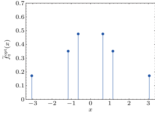
Fig. 5. Approximation of the optimal noise PDF using Eq. (20) with K = 3 Delta kernel functions. The parameters are given by [v_1, v_2, v_3, \mu_1, \mu_2, \mu_3]^T = [0.3512, 0.1723, 0.4765, 1.1609, 3.0505, 0.6393]^T .
